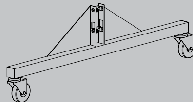
L-Leg with Casters, pg. 20
