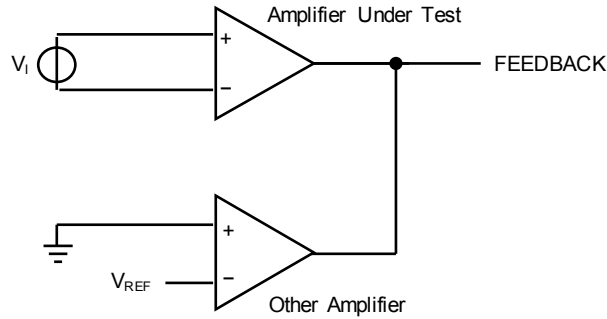
Fig 2. Amplifier Characteristics
